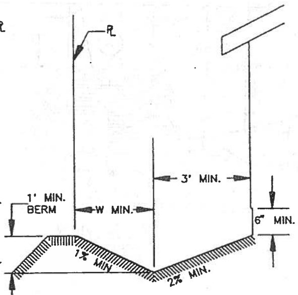
SECTION "A-A" SIDE YARD SWALE
