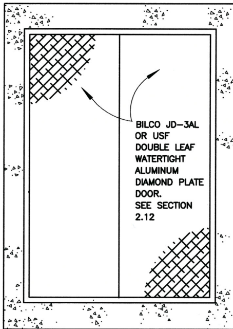
PLAN
