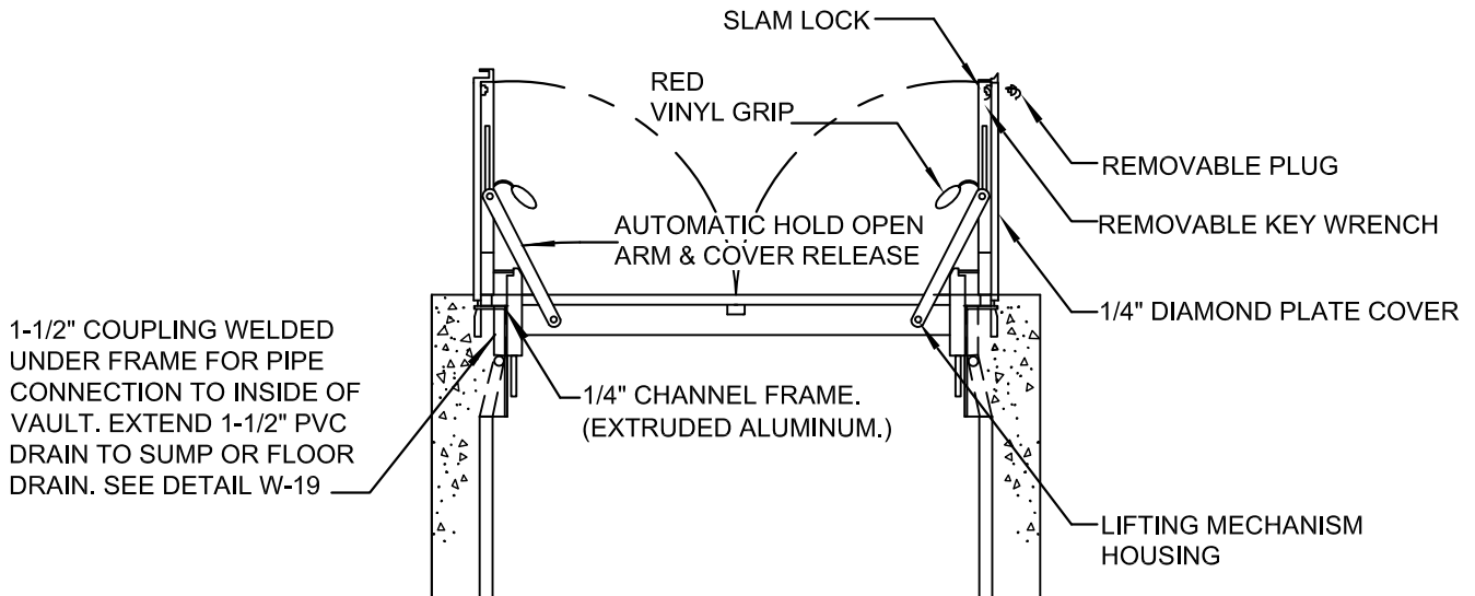
SECTION
