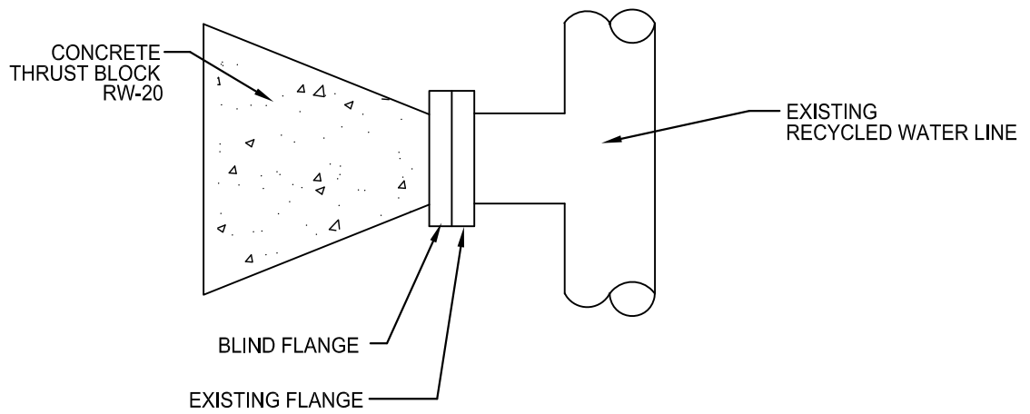
FLANGED OUTLET
